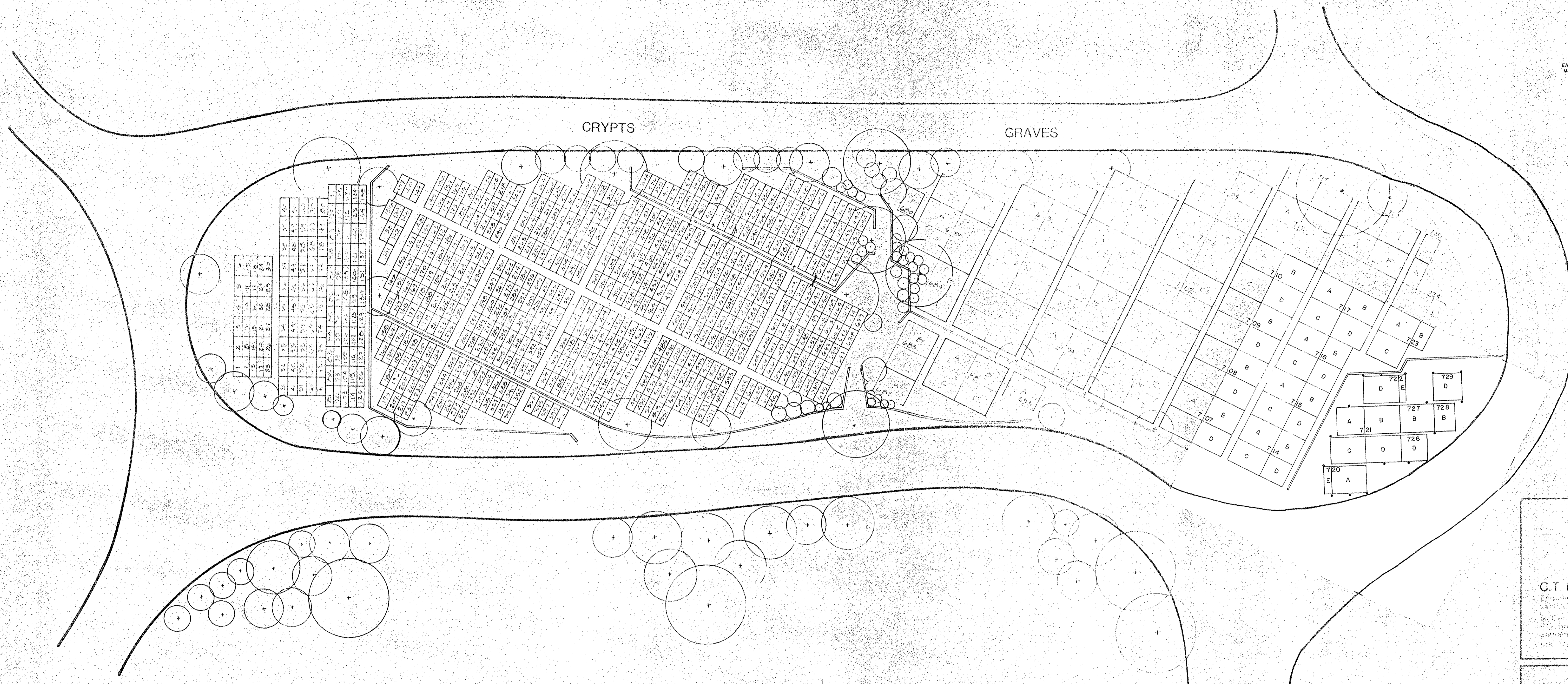
TYPICAL PLOT PLAN (LOTS 720-722 & 726-729) SCALE: 1"=10'
