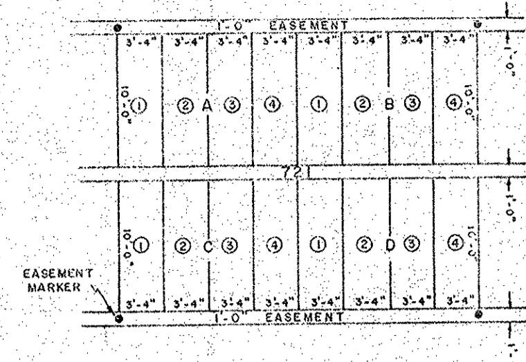
TYPICAL PLOT PLAN (LOTS 720-722 & 726-729) SCALE: 1"=10'
