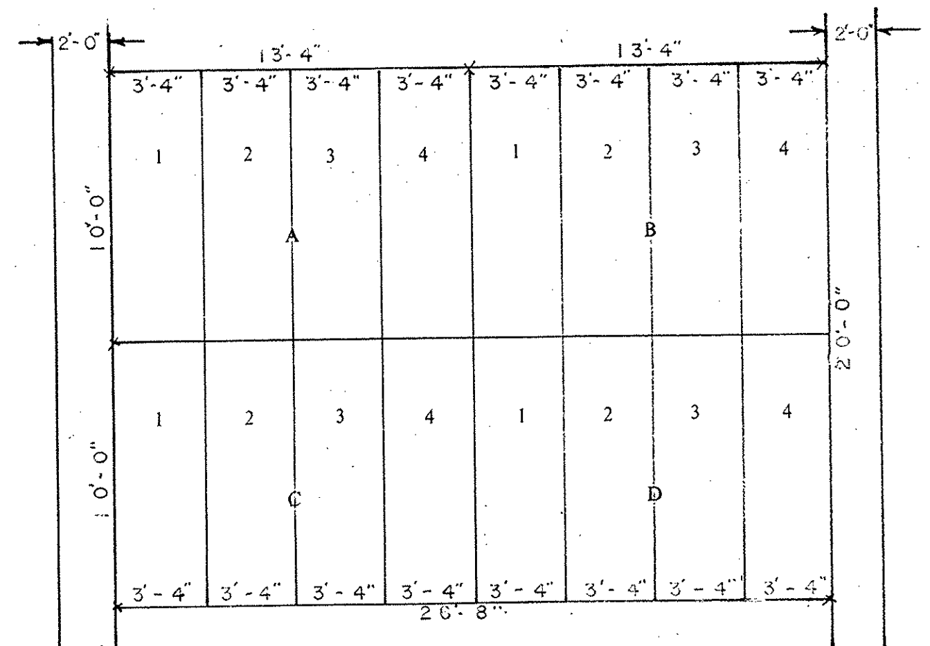
Typical Plot Plan Scale 1"=5'-0"
